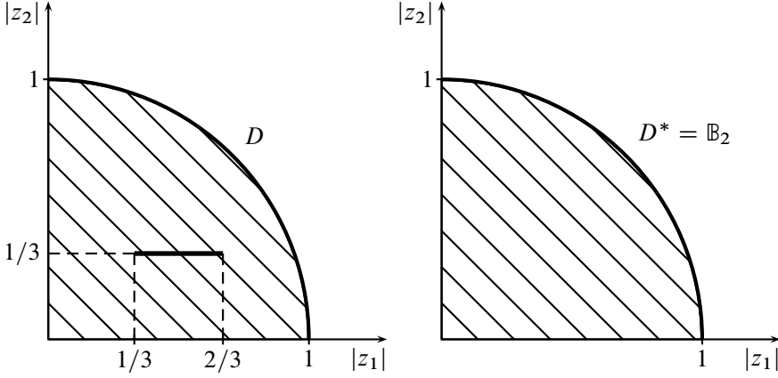
Figure 1.5.7. D := \mathbb{B}_2 \setminus \{(z_1, z_2) : 1/3 \leq |z_1| \leq 2/3, |z_2| = 1/3\} . If D is an arbitrary Reinhardt domain, then it may happen that D^* \setminus D \not\subset V_0 .
