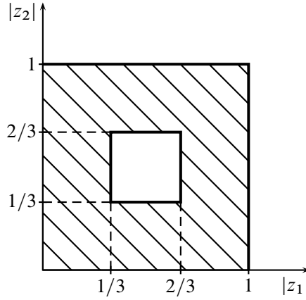
Figure 1.11.3. The domain D := \mathbb{D}^2 \setminus (\bar{\mathbb{A}}(1/3, 2/3) \times \bar{\mathbb{A}}(1/3, 2/3)) is weakly relatively complete, but not relatively complete.
