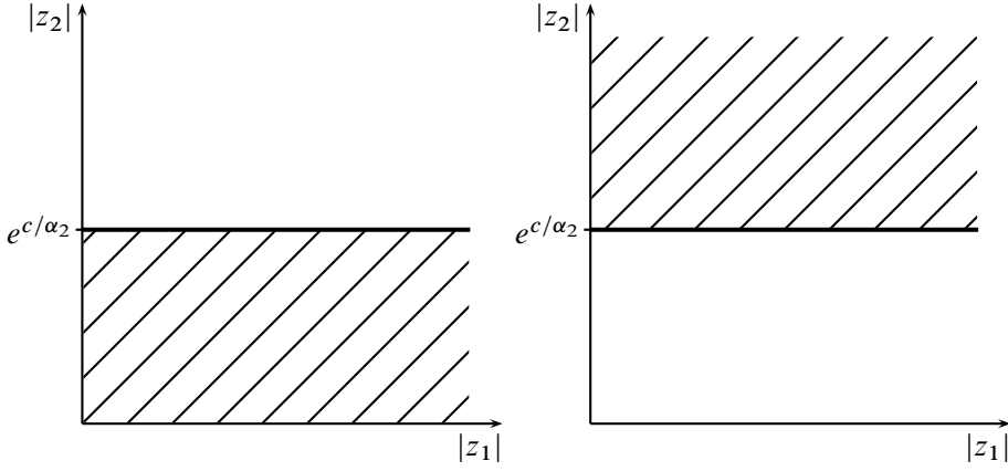
Figure 1.5.5. Elementary domains \mathbf{D}_{\alpha,c} with (\alpha_1 = 0, \alpha_2 > 0) and (\alpha_1 = 0, \alpha_2 < 0) .
